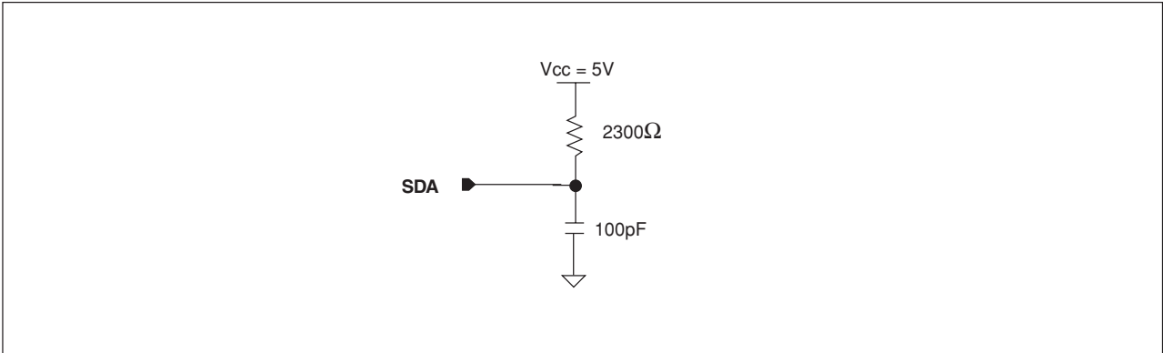
Figure 20. Equivalent A.C. Circuit
