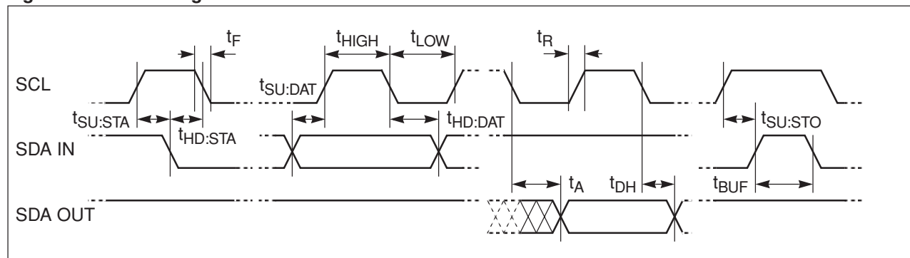
Figure 22. Bus Timing
