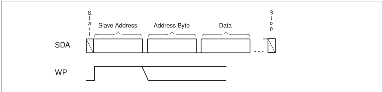
Figure 26. Write Protect (WP) Pin Timing
