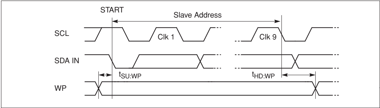
Figure 25. Write Protect (WP) Pin Timing During Slave Address
