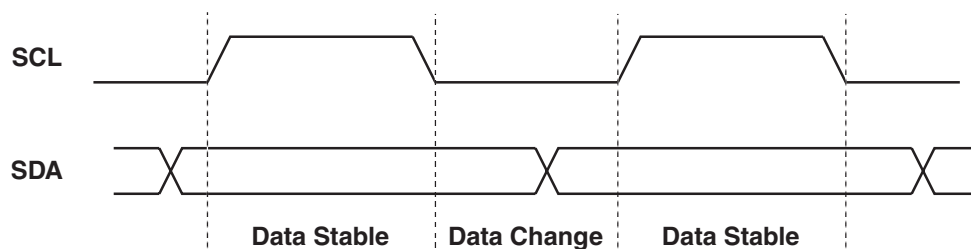
Figure 1. Valid Data Changes on the SDA Bus
