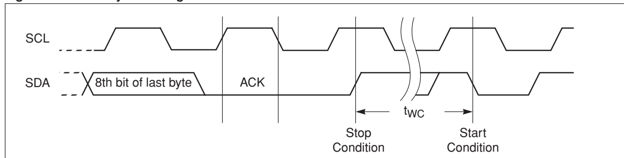
Figure 24. Write Cycle Timing
