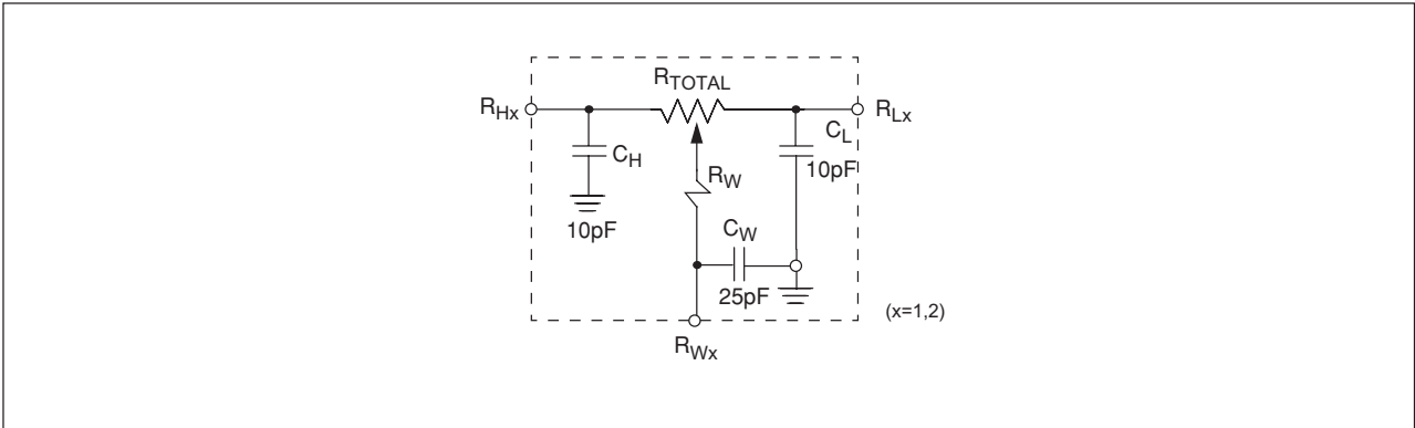
Figure 21. DCP SPICE Macromodel
