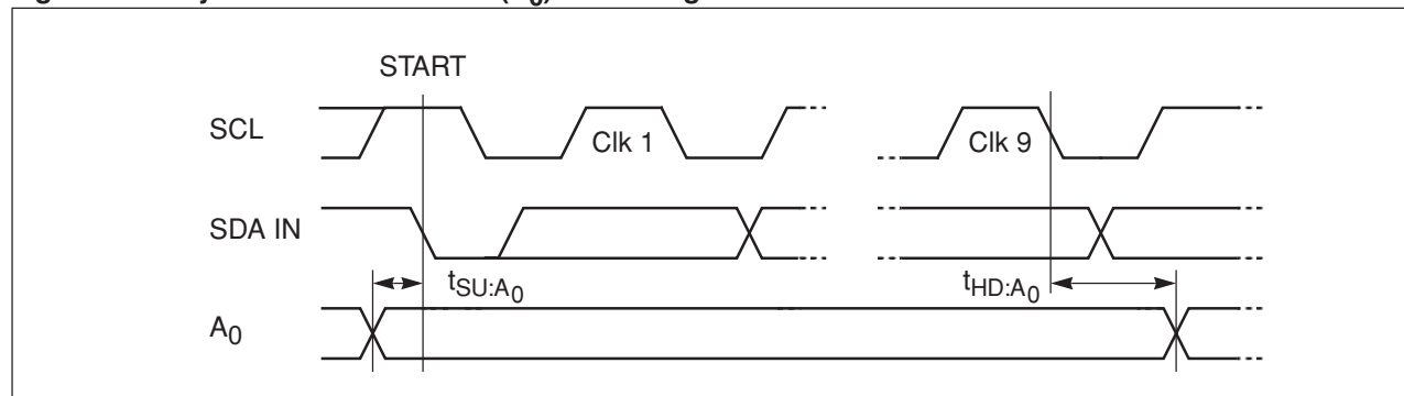
Figure 23. Physical Device Address ( A_0 ) Pin Timing
