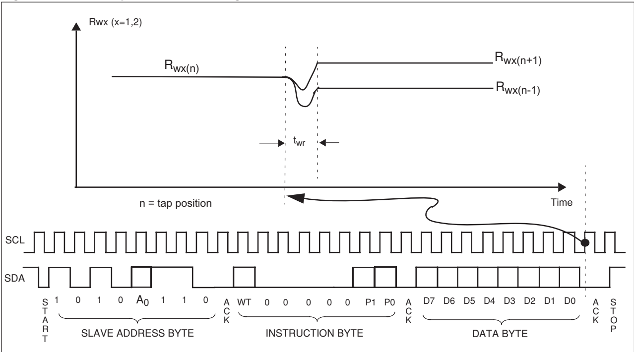
Figure 27. DCP “Wiper Position” Timing
