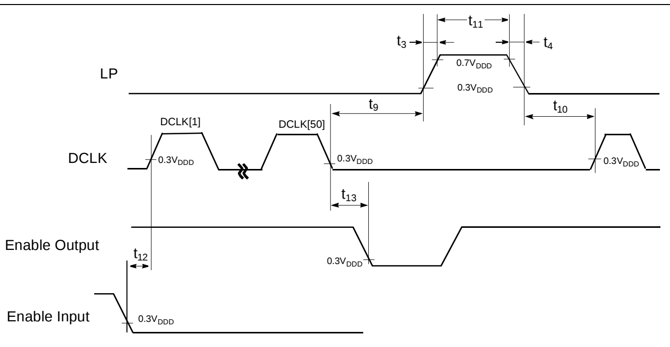
Figure 5-4: LP, DCLK, EIO1#and EIO300# Timing Relationship (2xCLK high)
