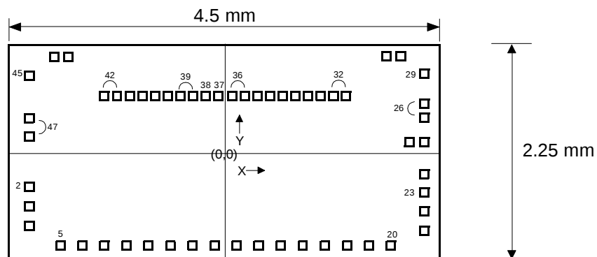
Figure 2-2: WFP6131AR Die
