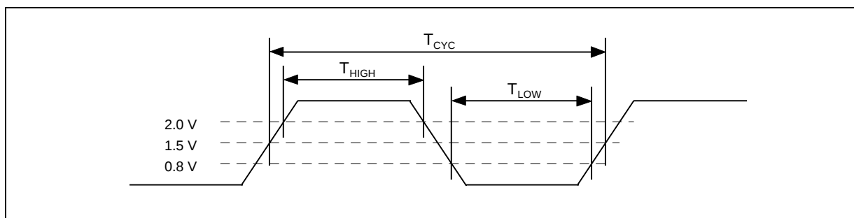
Figure 9.6 Clock Waveform
