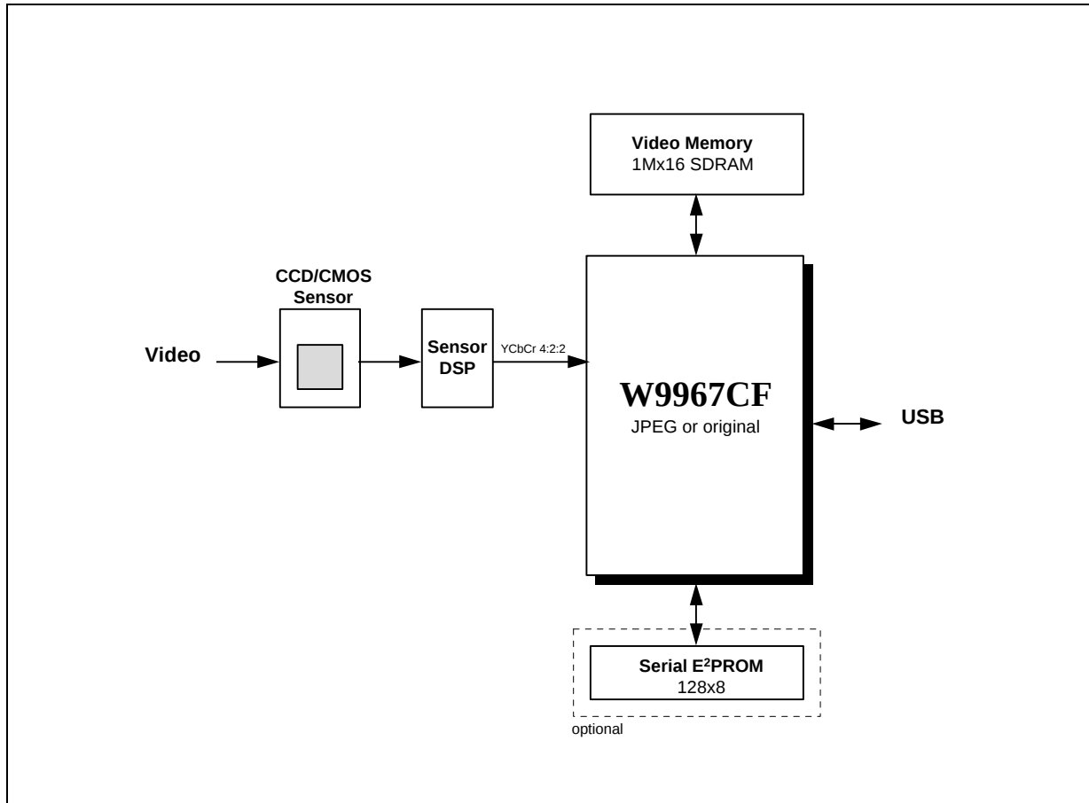
Figure 5.1 W9967CF-Based USB Digital Video Camera System Diagram
