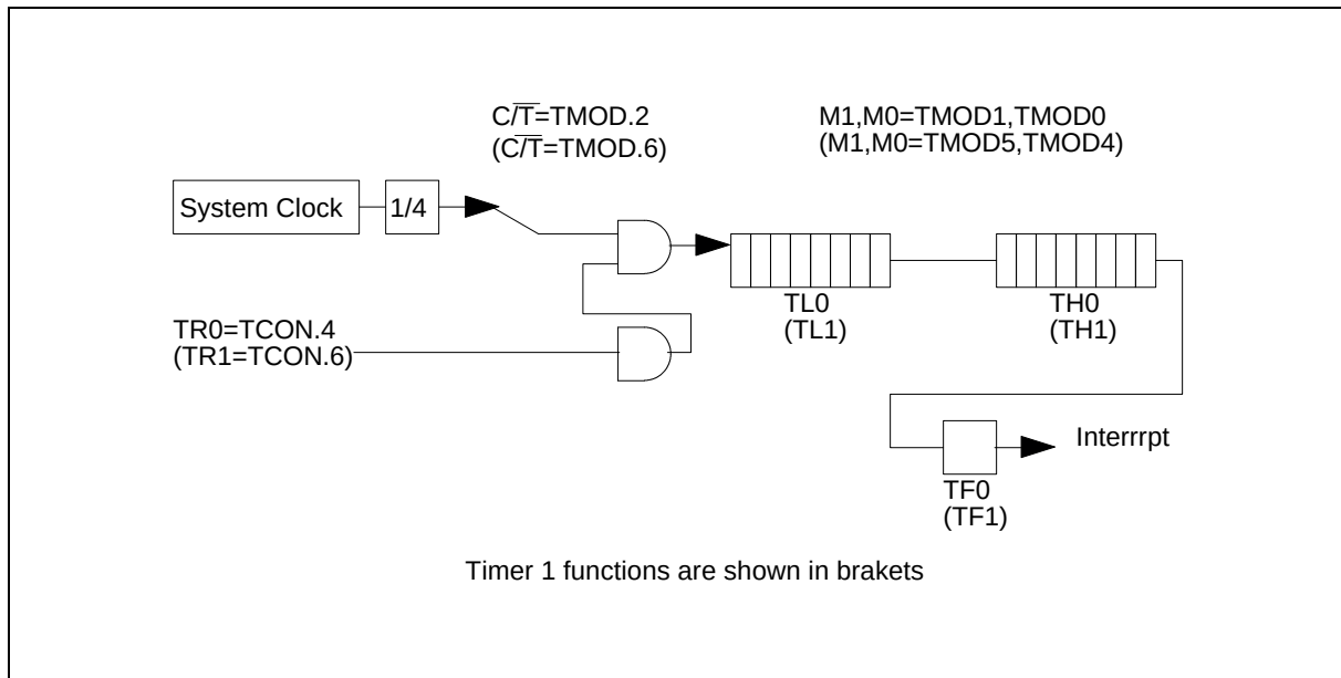
Mode 1 of Timer 0 & 1
