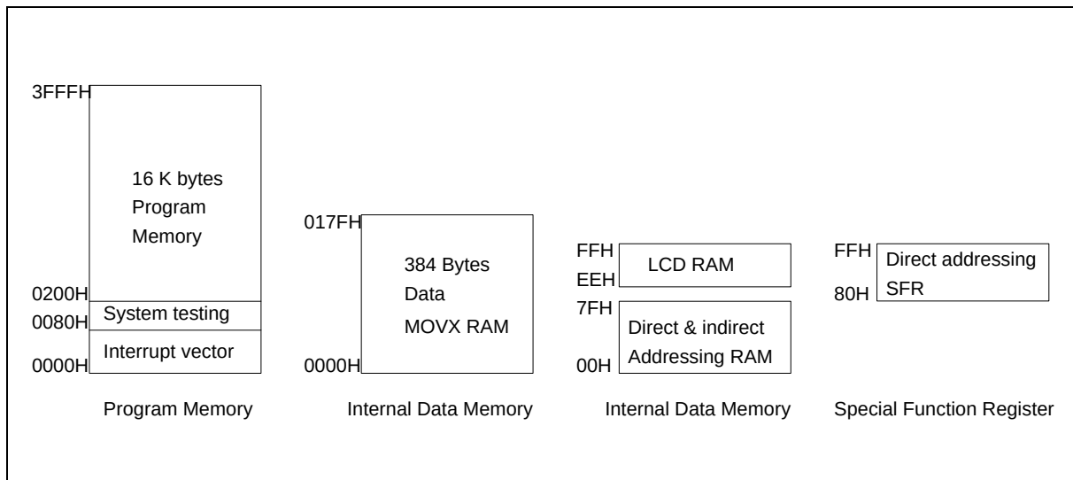
On-chip memory space of W928C70
