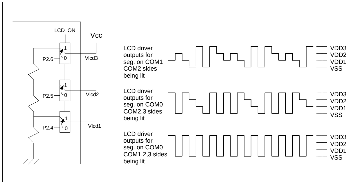
LCD Voltage Pin Connection and Output Waveform (1/3 Bias 1/4 Duty)
