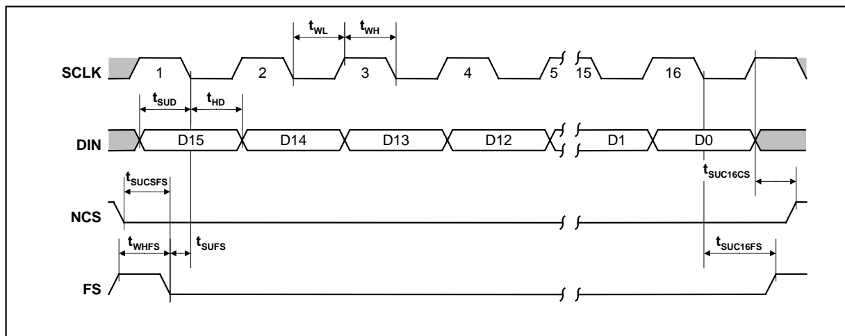
Figure 1 Timing Diagram
