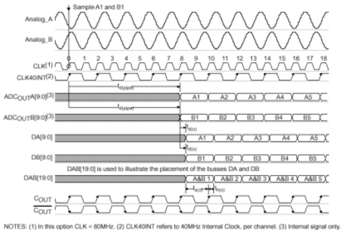
Figure 1 Timing Diagram, Dual Bus Output - Option 1
