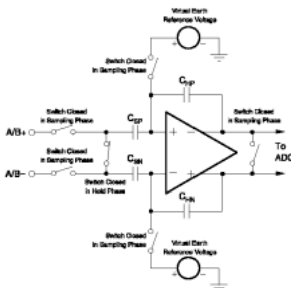
Figure 6. SHA/SHPGA Architecture
