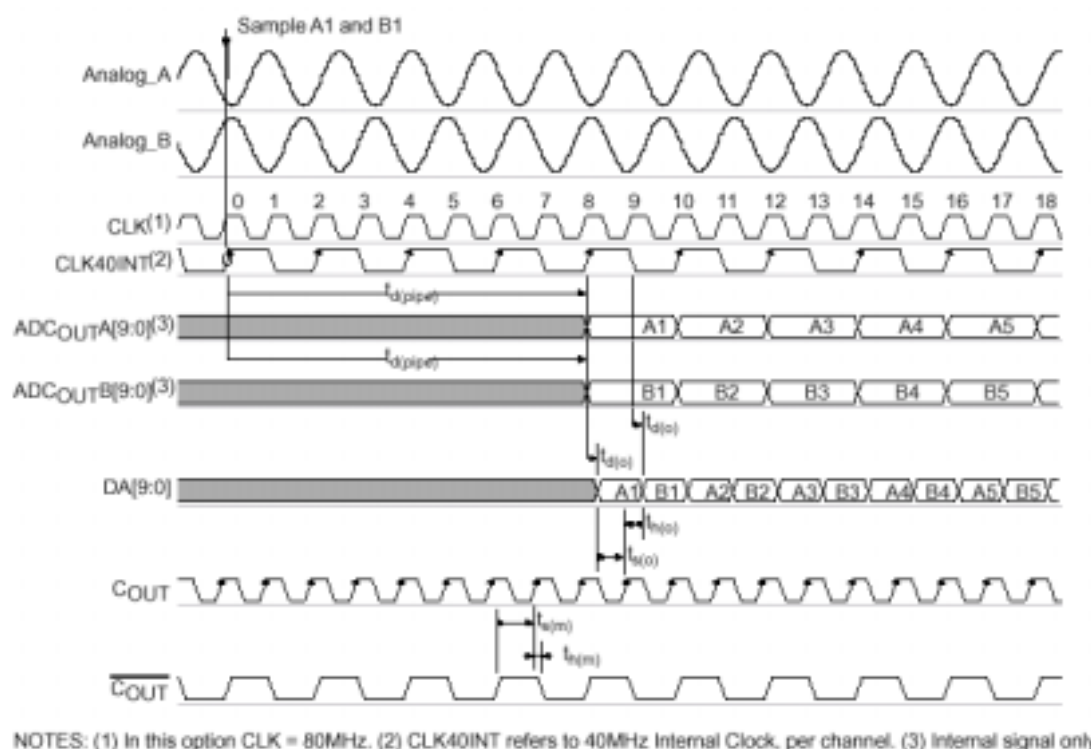
Figure 4 Timing Diagram, Single Bus Output - Option 2
