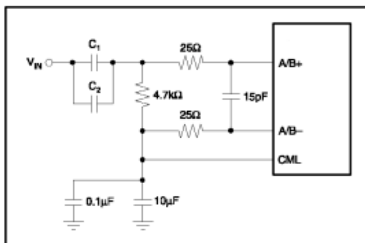
Figure 10 AC-Coupled, Single-Ended Configuration
