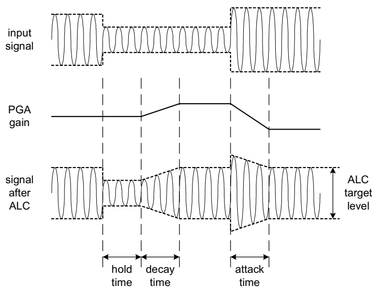
Figure 21 ALC Operation
