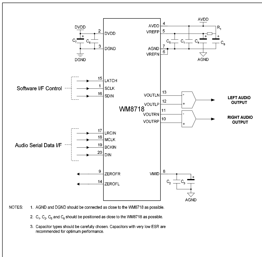
Figure 23 External Components Diagram
