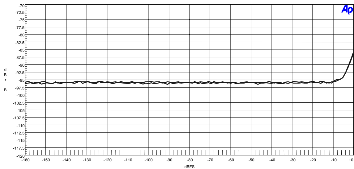
Figure 9 WM8762 Functionality THD+N VDD = 3V
