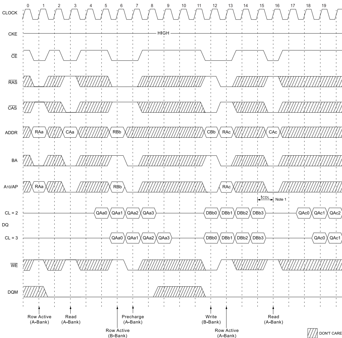
FIG. 9 READ &amp; WRITE CYCLE AT DIFFERENT BANK @BURST LENGTH=4
