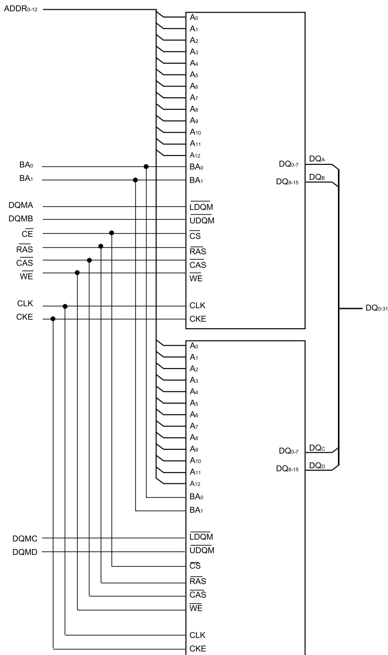
FIG. 2 16MX32 SDRAM BLOCK DIAGRAM
