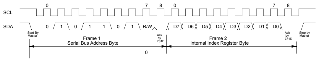
Figure 3. Serial Bus Write to Internal Address Register Only
