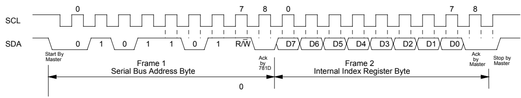
Figure 4. Serial Bus Write to Internal Address Register Only
