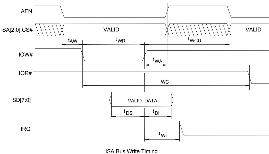
ISA Read/Write Timing
