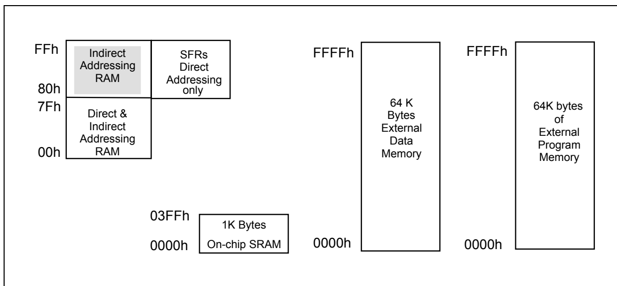
Figure 1. Memory Map
