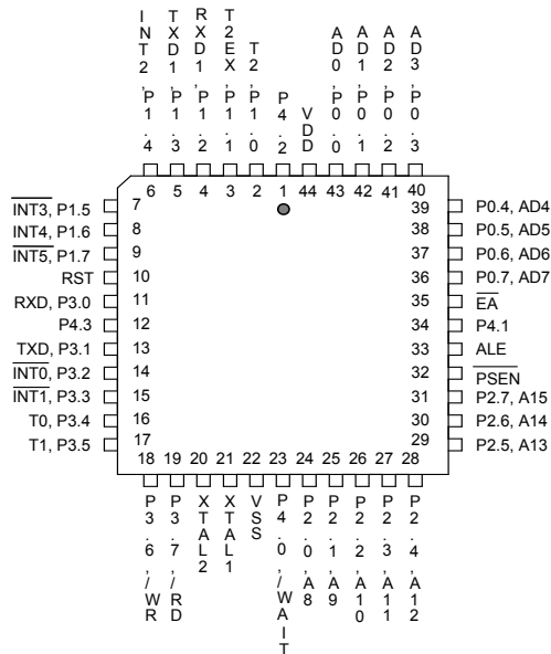
44-Pin PLCC
