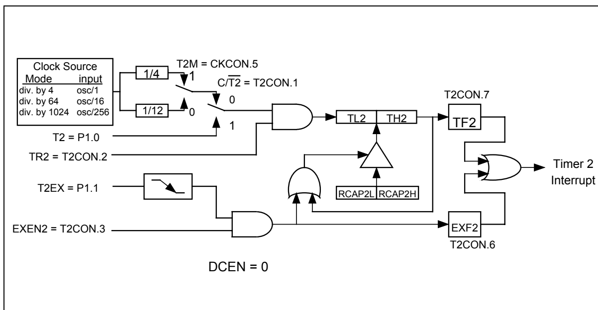
Figure 15. 16-Bit Auto-reload Mode, Counting Up
