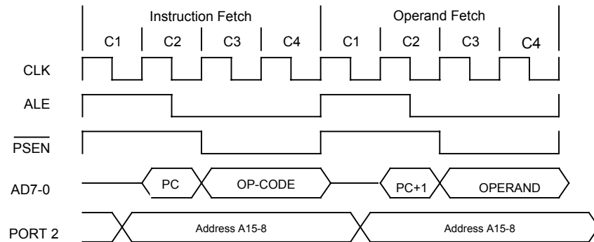
Figure 4: Two Cycle Instruction Timing
