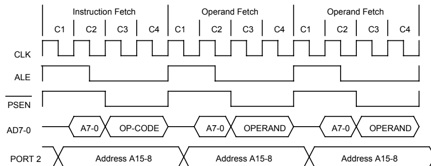
Figure 5: Three Cycle Instruction Timing
