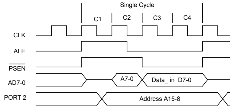
Figure 3: Single Cycle Instruction Timing
