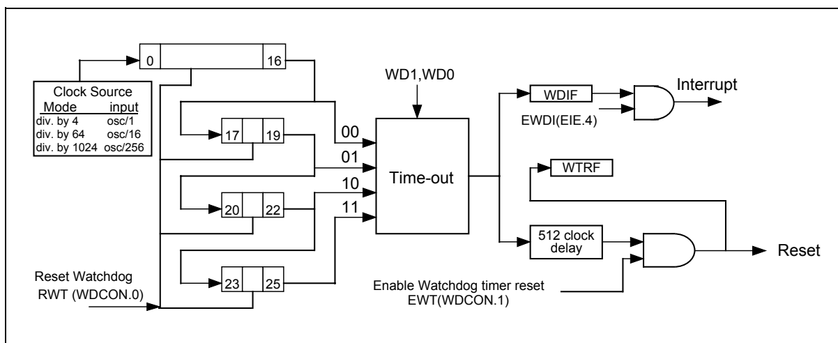
Figure 19. Watchdog Timer
