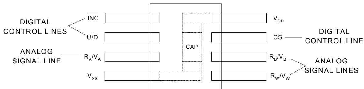
FIGURE 9 – WMS7140/7141 LAYOUT
