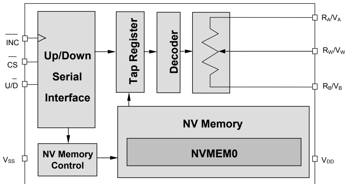
FIGURE 1 – WMS7120 BLOCK DIAGRAM (Rheostat/Divider Mode)
