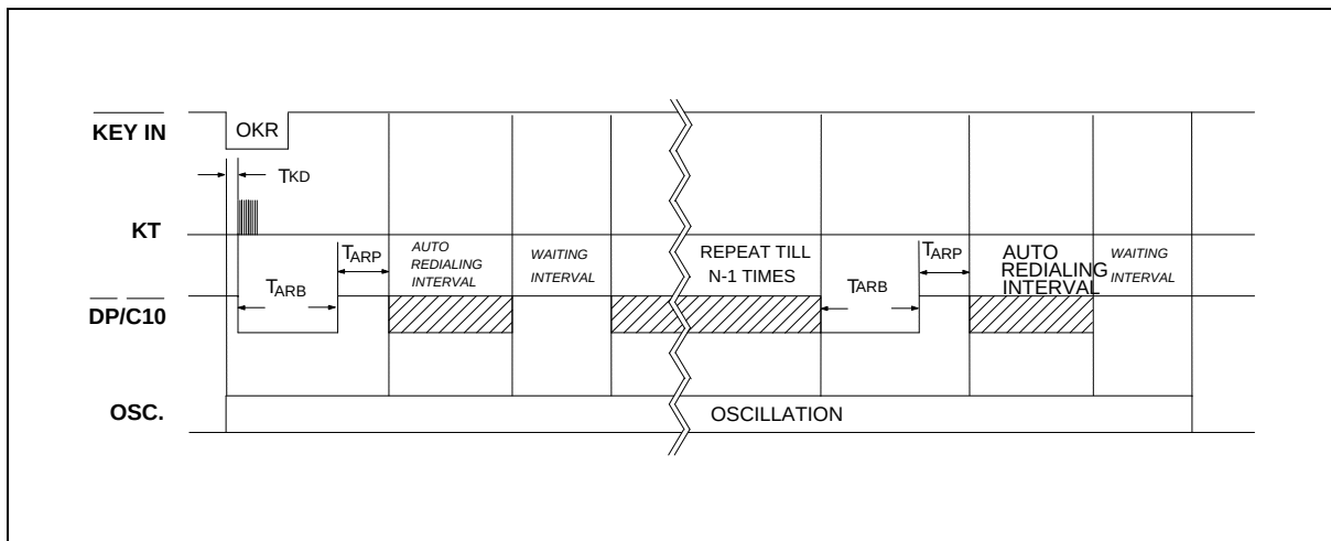
Figure 11(a). Auto Redialing Timing Diagram
