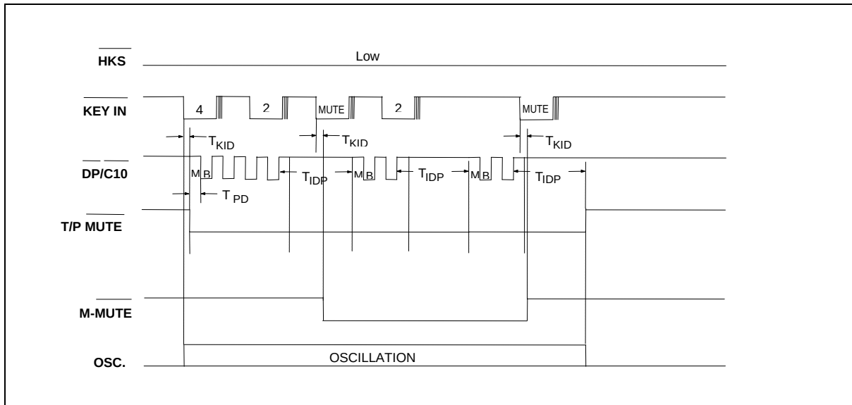
Figure 9. Mute Timing Diagram
