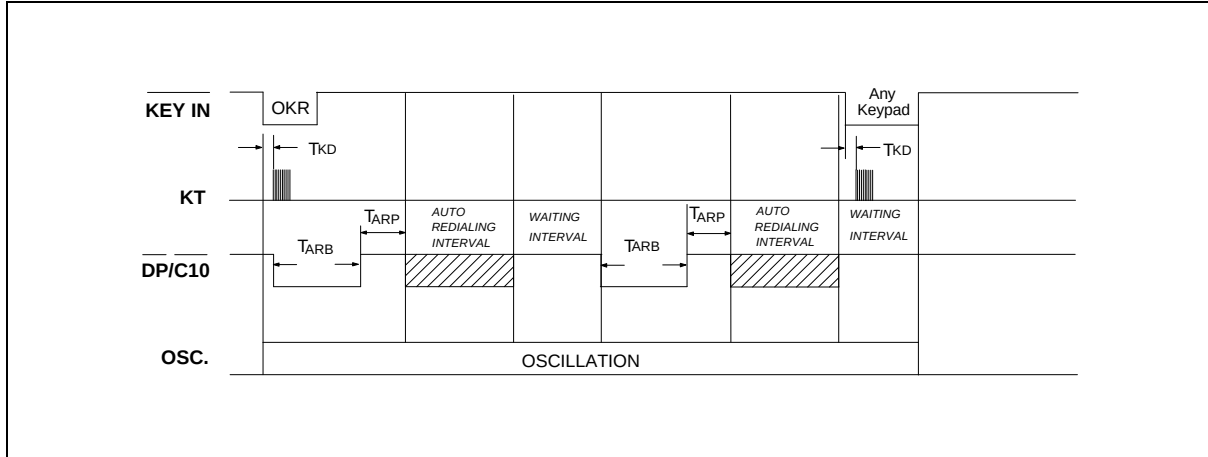
Figure 11(b). Auto Redialing Timing Diagram
