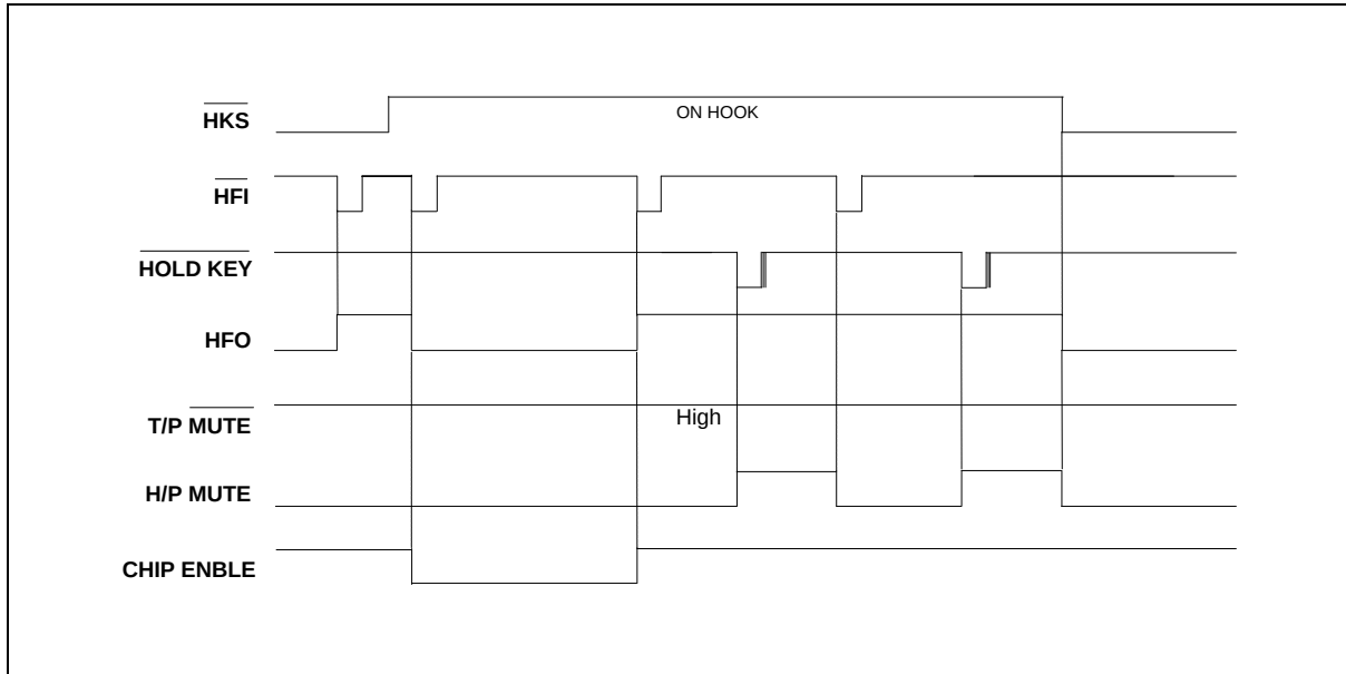
Figure 10(c). Hold and Handfree Timing Diagram
