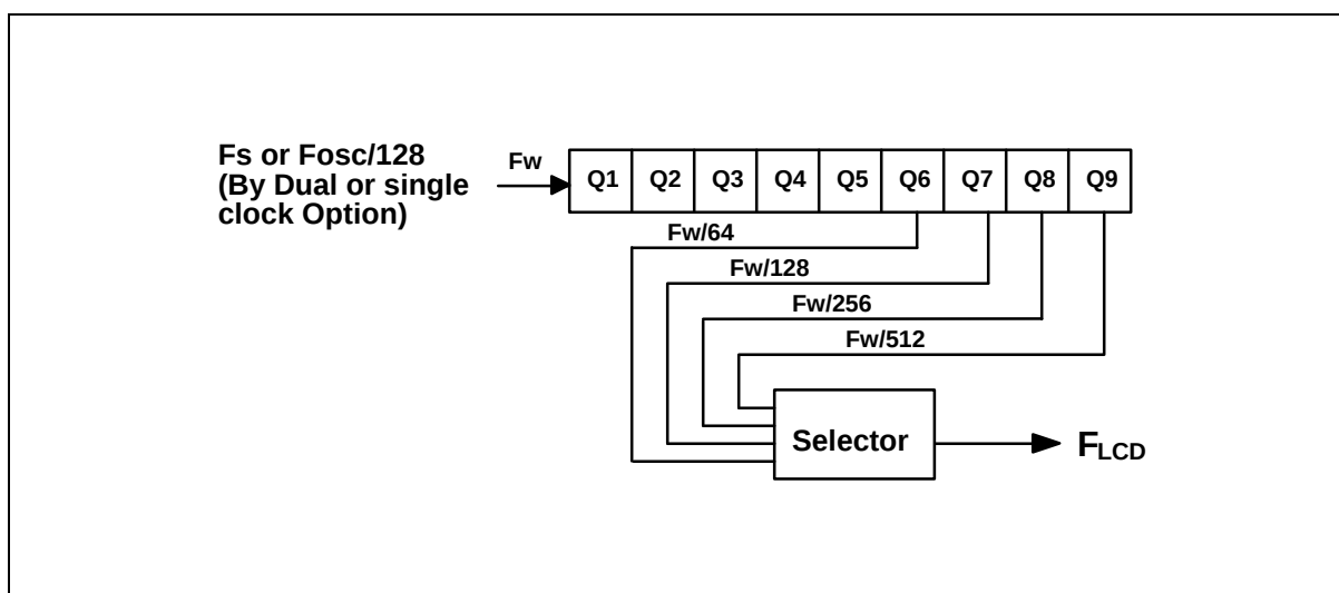
Figure 6-14 LCD alternating frequency (FLCD) circuit diagram
