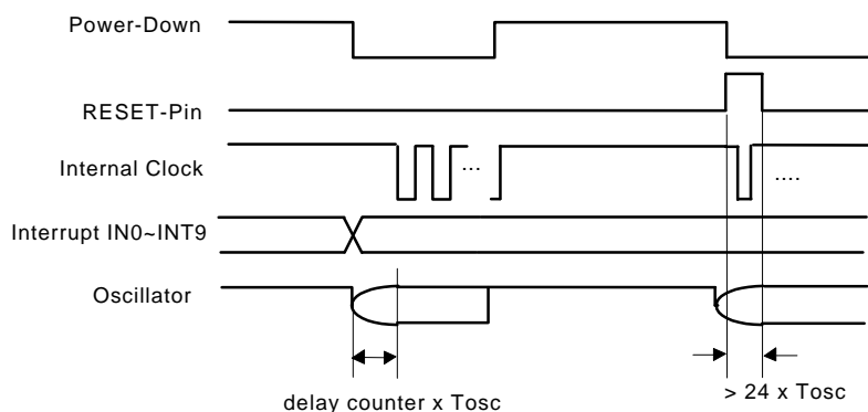
Fig. Power-Down Wake Up Operation
