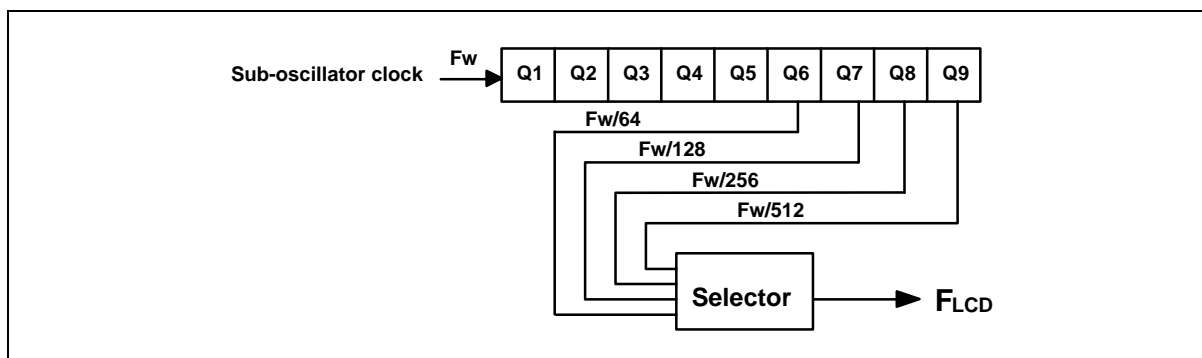
Figure 6-14 LCD alternating frequency (FLCD) circuit diagram
