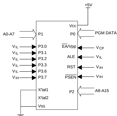
Programming Configuration
