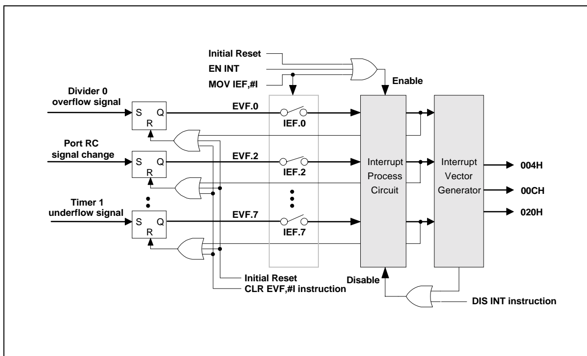
Figure 6. Interrupt Event Control Diagram
