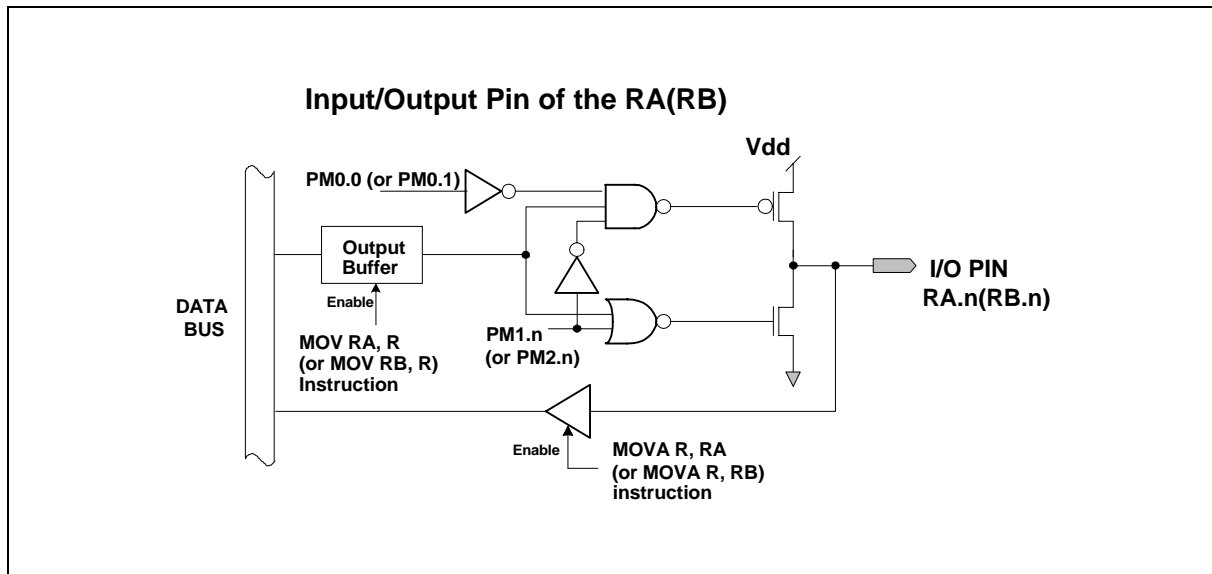
Figure 8. Architecture of Input/Output Pins
