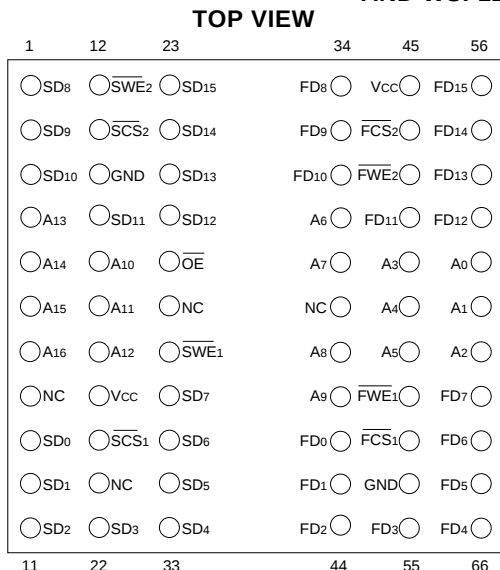
FIG. 1 PIN CONFIGURATION FOR WSF128K16-XXH AND WSF128K16-XH1X
