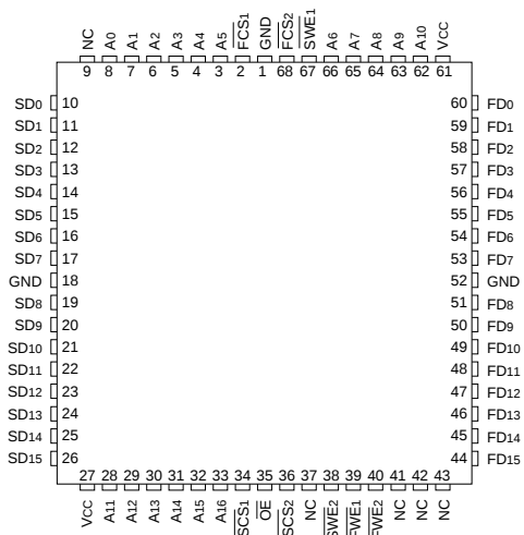
FIG. 2 PIN CONFIGURATION FOR WSF128K16-XG1UX
