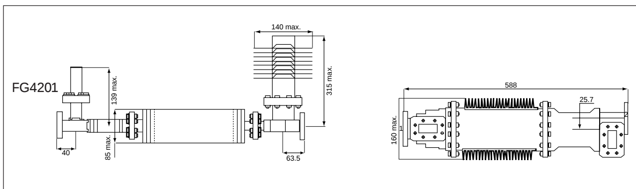
R48 WR187 waveguide
