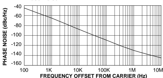
Phase Noise
