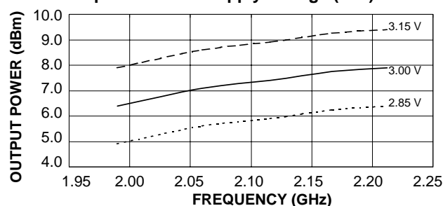
Output Power vs Supply Voltage ( V_{CC} )
