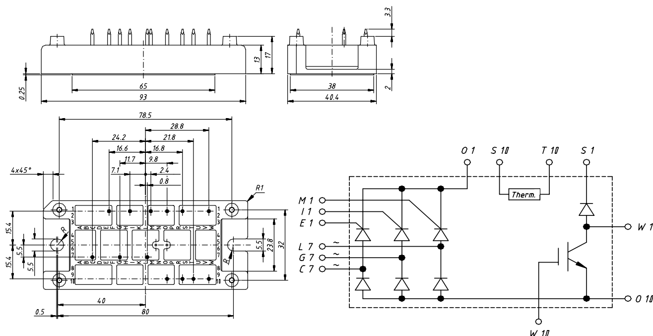
Dimensions in mm (1 mm = 0.0394")
