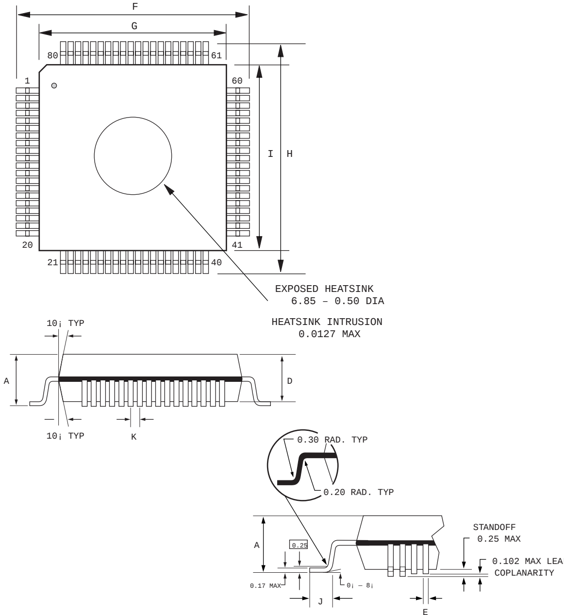
80-Pin PQFP Package Drawing
