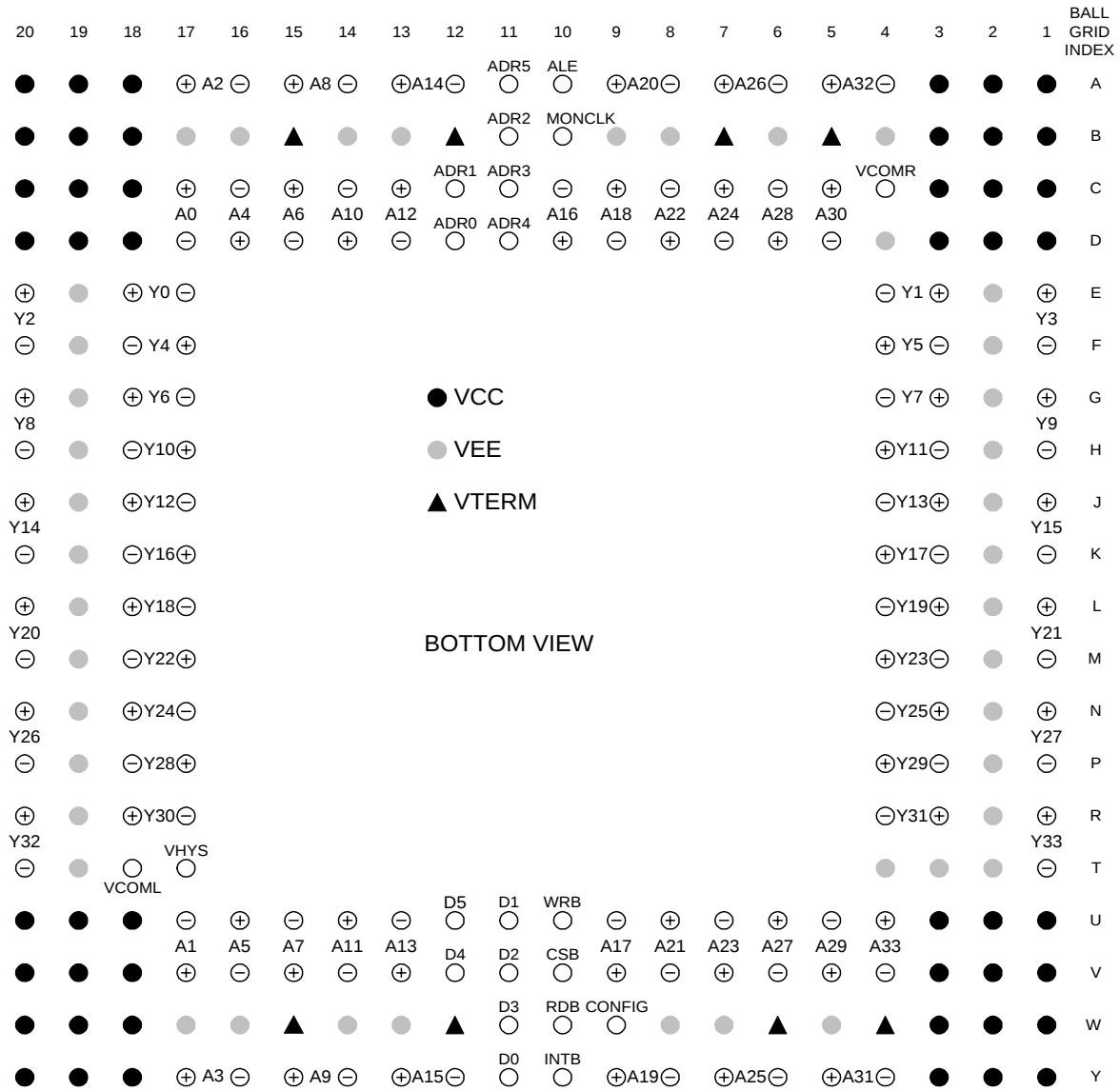
Figure 7: Pinout Diagram
