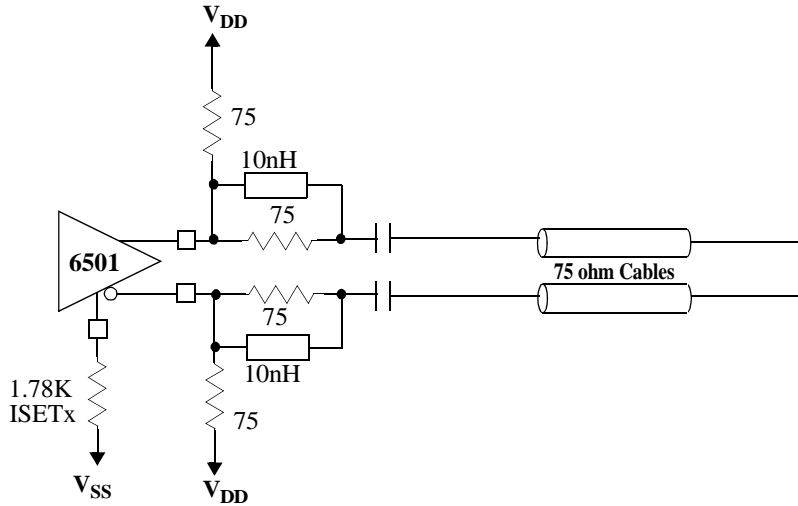
Figure 1: High Speed Interconnect Example (Differential)
