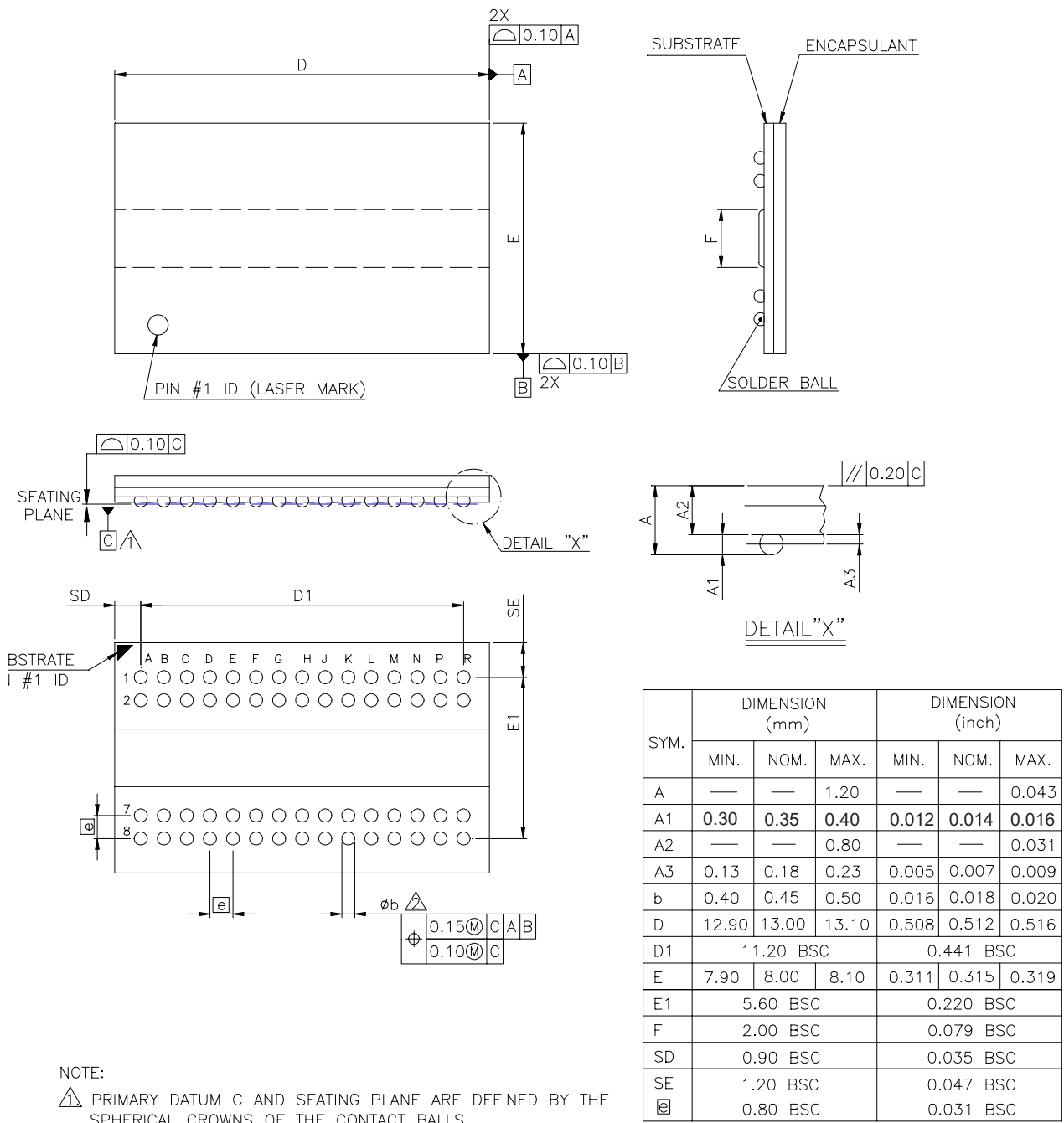
Package Diagram 60 Ball SOC BGA
