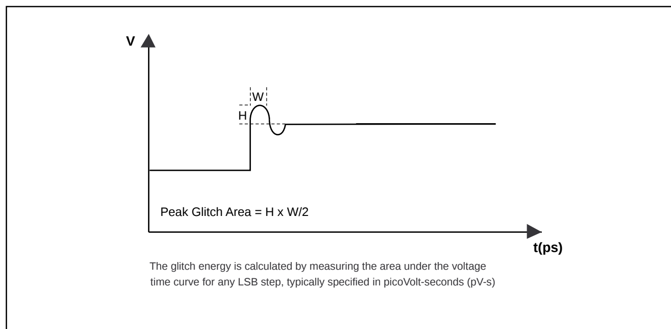
Figure 3 Glitch Energy
