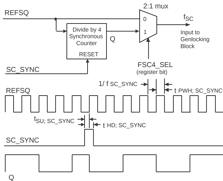
Figure 5 REFSQ and SC_SYNC input timing
