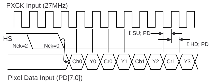
Figure 4 REC 656 interface with HS output timing
