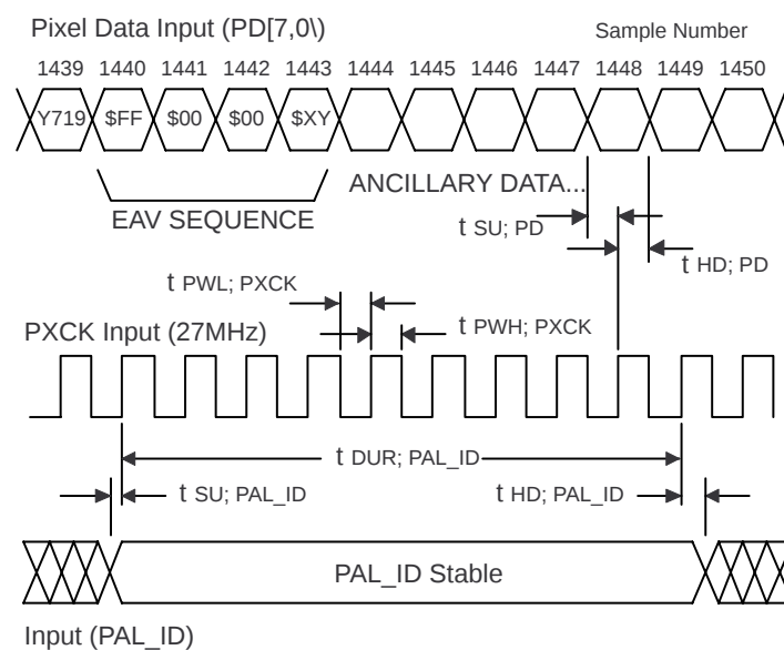
Figure 6 PAL_ID input timing
