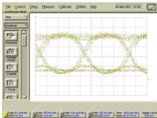
Eye Diagram at 2.5 Gbps
