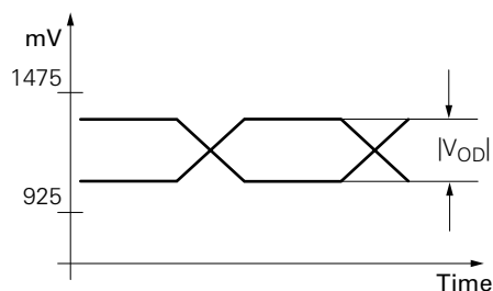
Figure 7. Output level diagram
