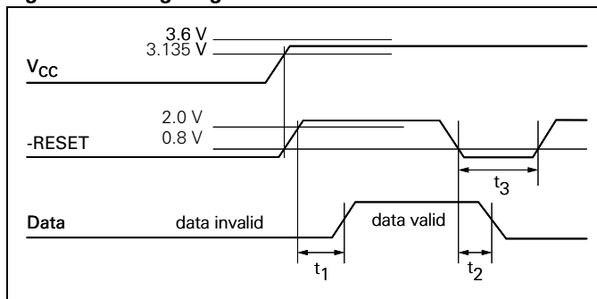
Figure 5. Timing diagram
