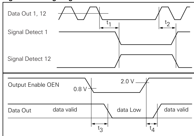
Figure 8. Timing diagrams
