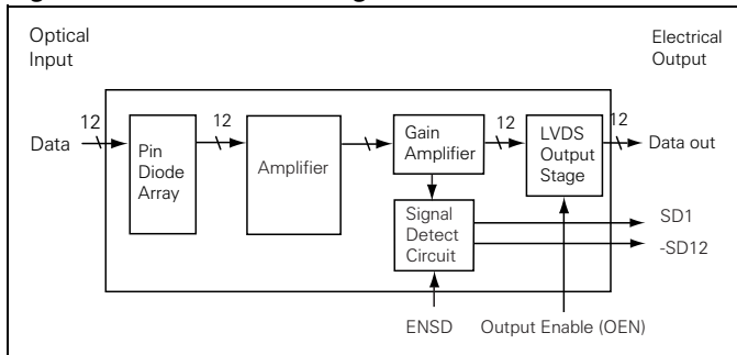
Figure 6. Receiver block diagram
