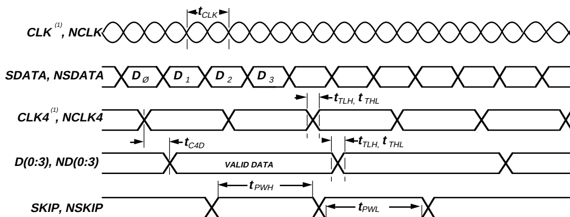
Figure 4: VS8005 Waveforms
