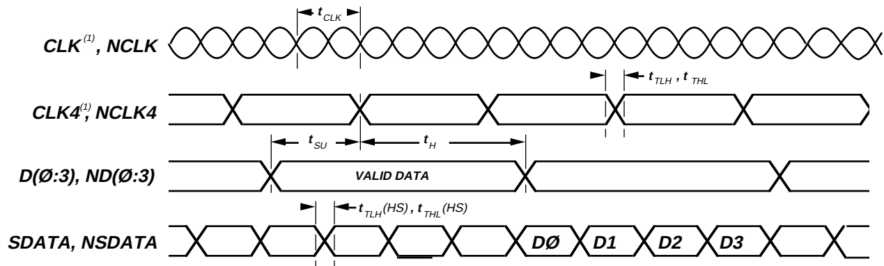
Figure 3: VS8004 Waveforms
