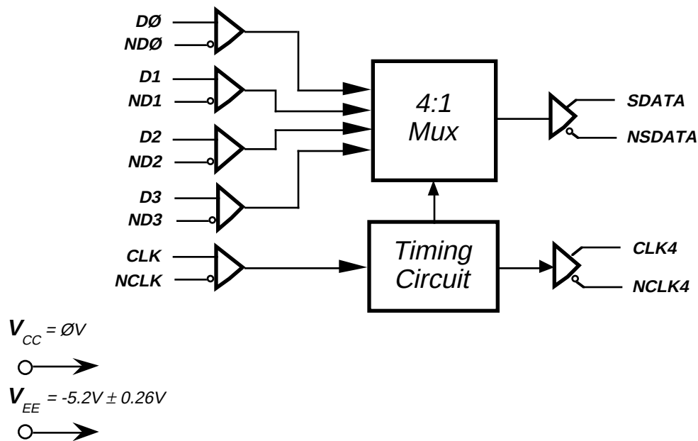
Figure 2: VS8005 Block Diagram
