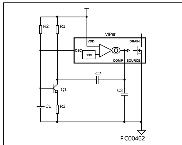
Figure 16: Slope Compensation
