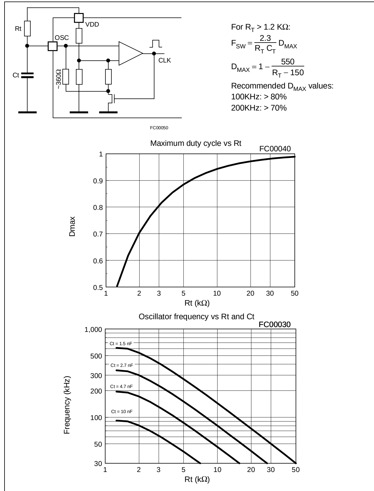
Figure 7: Oscillator
