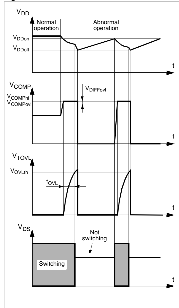
Figure 4: Overload event
