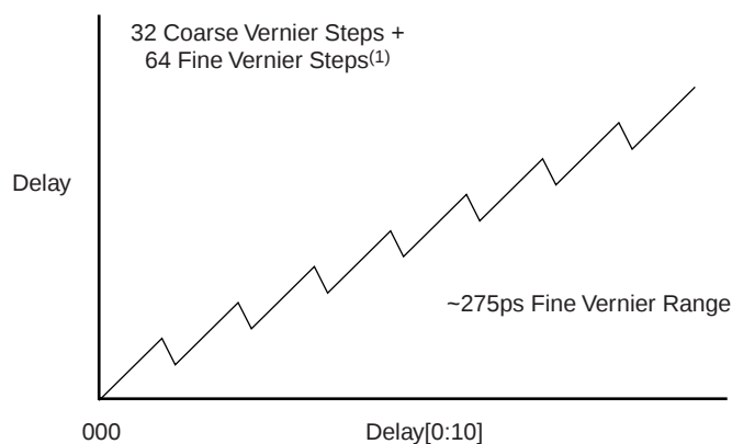
Figure 5: CAL Mode: Pre-Calibration Delay Range
