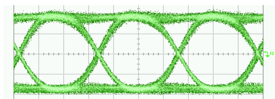
3.125Gbps eye diagram
