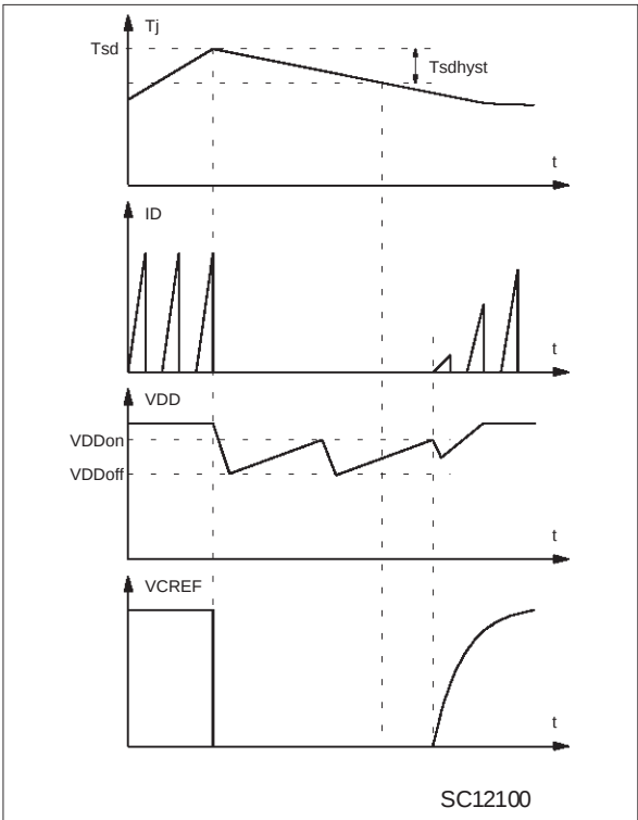
Figure 8: Overtemperature Protection
