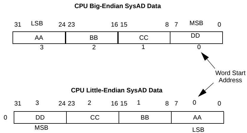
Figure 15. Bit and Byte Order of Endian Modes (Word Accesses)
