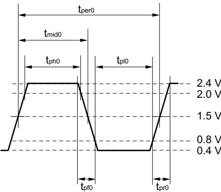
Figure 62. PCI CLK Input Waveform at Destinations
