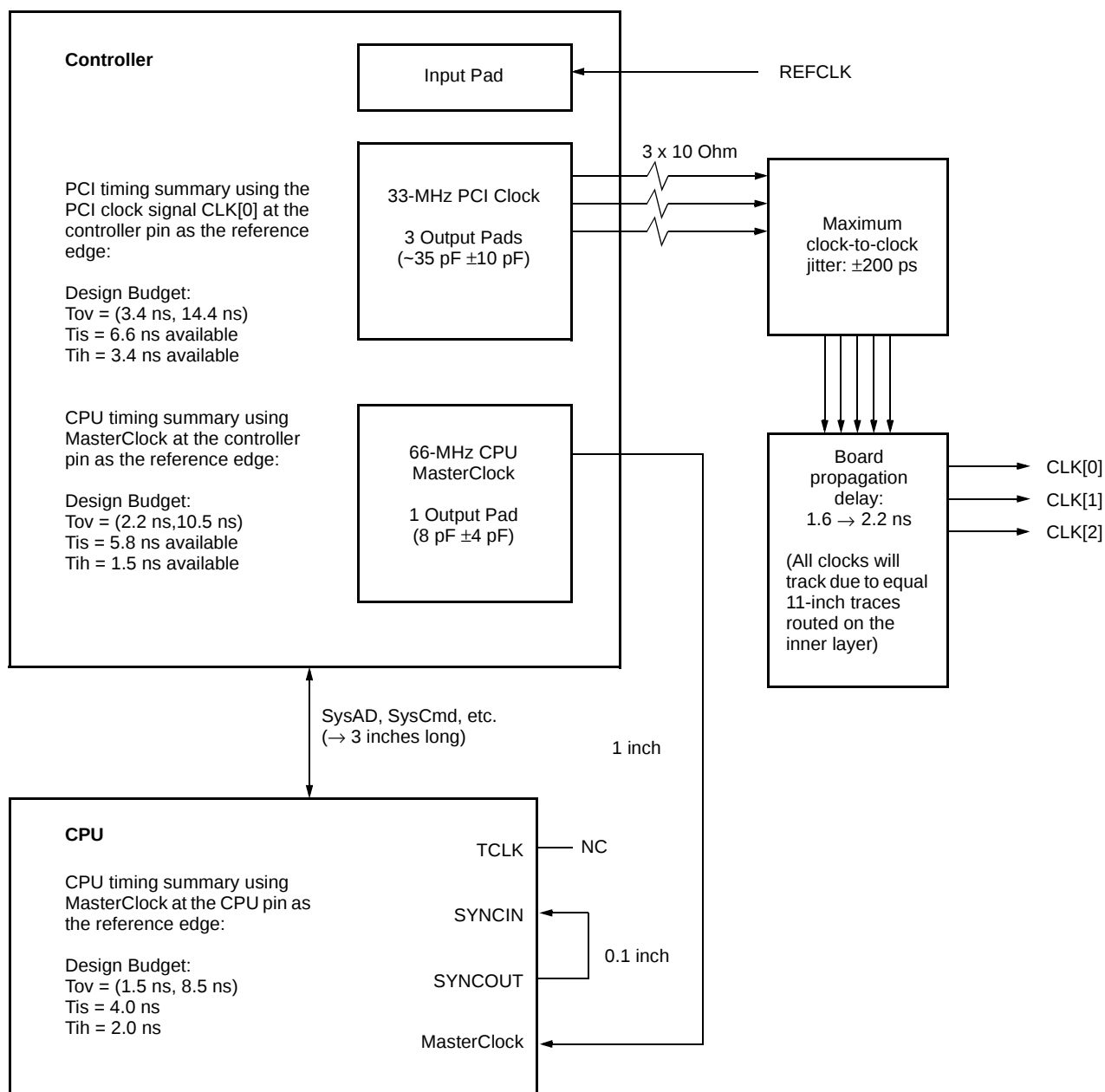
Figure 11. Clock Connections
