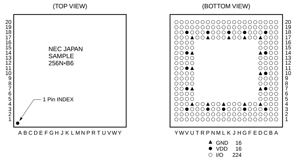
Figure 2. Pin Configuration
