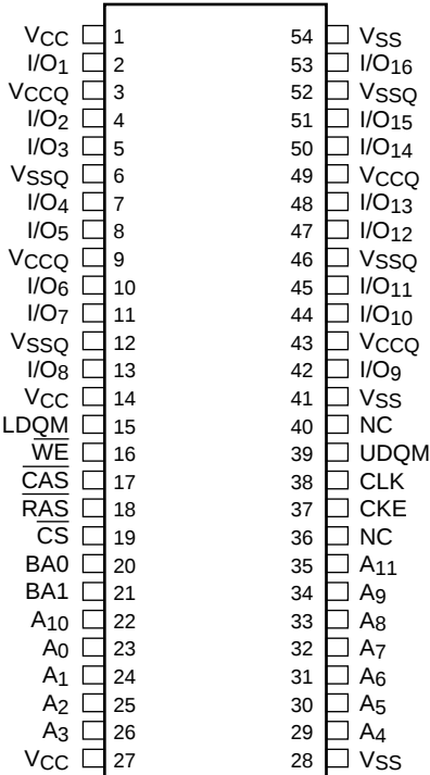
54 Pin Plastic TSOP-II PIN CONFIGURATION Top View
