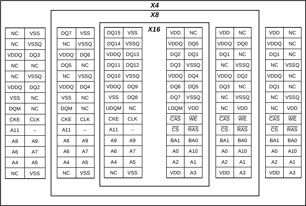
WBGA SDRAM (X4/X8/X16) 56 PINS ASSIGNMENT (Top View)
