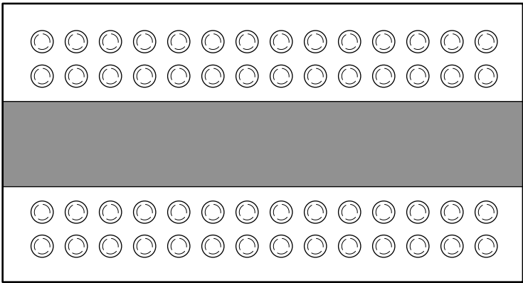
WBGA SDRAM (X4/X8/X16) 56 PINS ASSIGNMENT (Top View)
