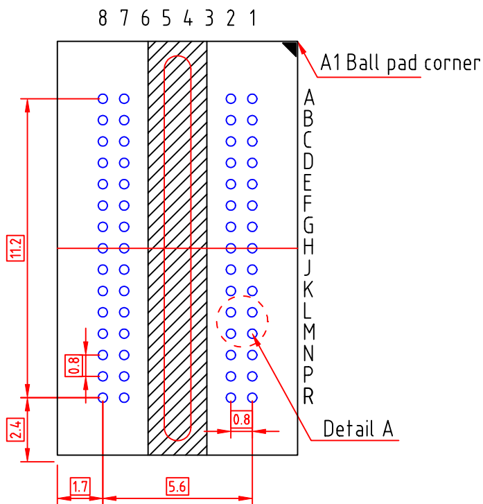
BOTTOM VIEW ( BALL SIDE )
