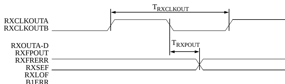
Figure 19: VSC8024 Parallel Data Output Timing Diagram
