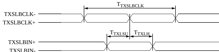
Figure 8: VSC8023 Serial Data Input Timing Diagram (Facility Loopback)
