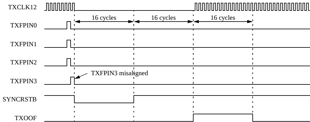
Figure 3: VSC8023 Synchronous Reset Timing Diagram
