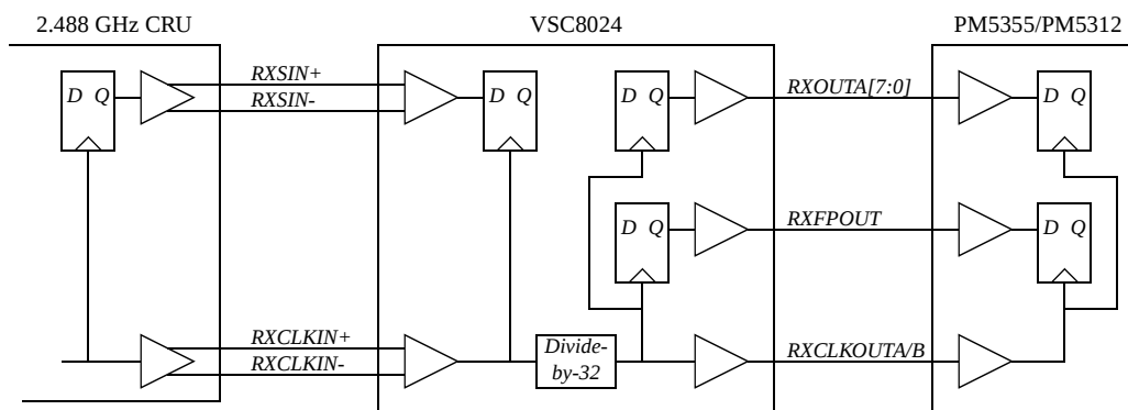
Figure 15: VSC8024 Clock and Data Interface Block Diagram (Serial Receive Mode)
