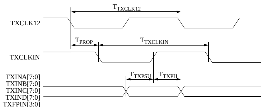
Figure 6: VSC8023 Parallel Data Input Timing Diagram
