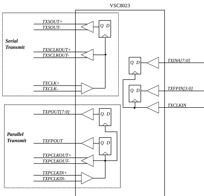
Figure 4: VSC8023 Clock and Data Interface (Serial Transmit & Parallel Transmit Mode)
