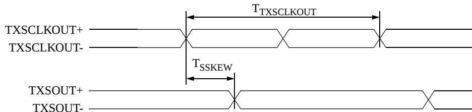
Figure 7: VSC8023 Serial Data Output Timing Diagram
