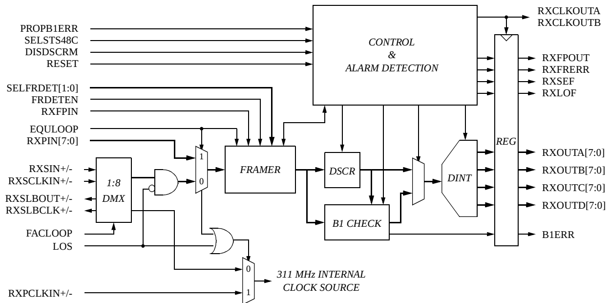
Figure 10: VSC8024 Functional Block Diagram
