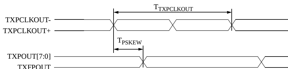
Figure 9: VSC8023 Parallel Data Output Timing Diagram (Equipment Loopback)
