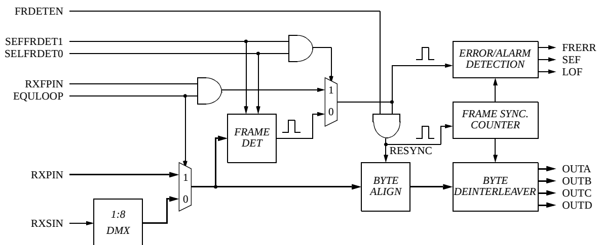
Figure 12: VSC8024 Functional Block Diagram of Frame Acquisition Circuit
