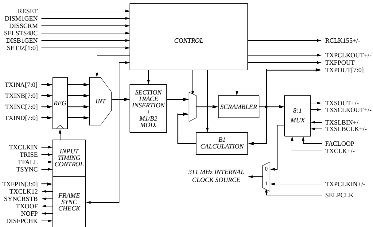
Figure 1: VSC8023 Functional Block Diagram
