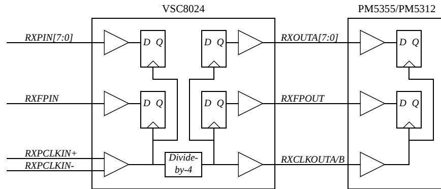
Figure 16: VSC8024 Clock and Data Interface Block Diagram (Parallel Receive Mode)
