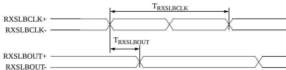
Figure 20: VSC8024 Serial Data Output Timing Diagram (Facility Loopback)
