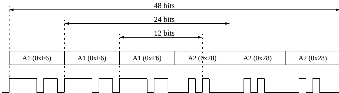
Figure 11: VSC8024 Frame Detection Patterns
