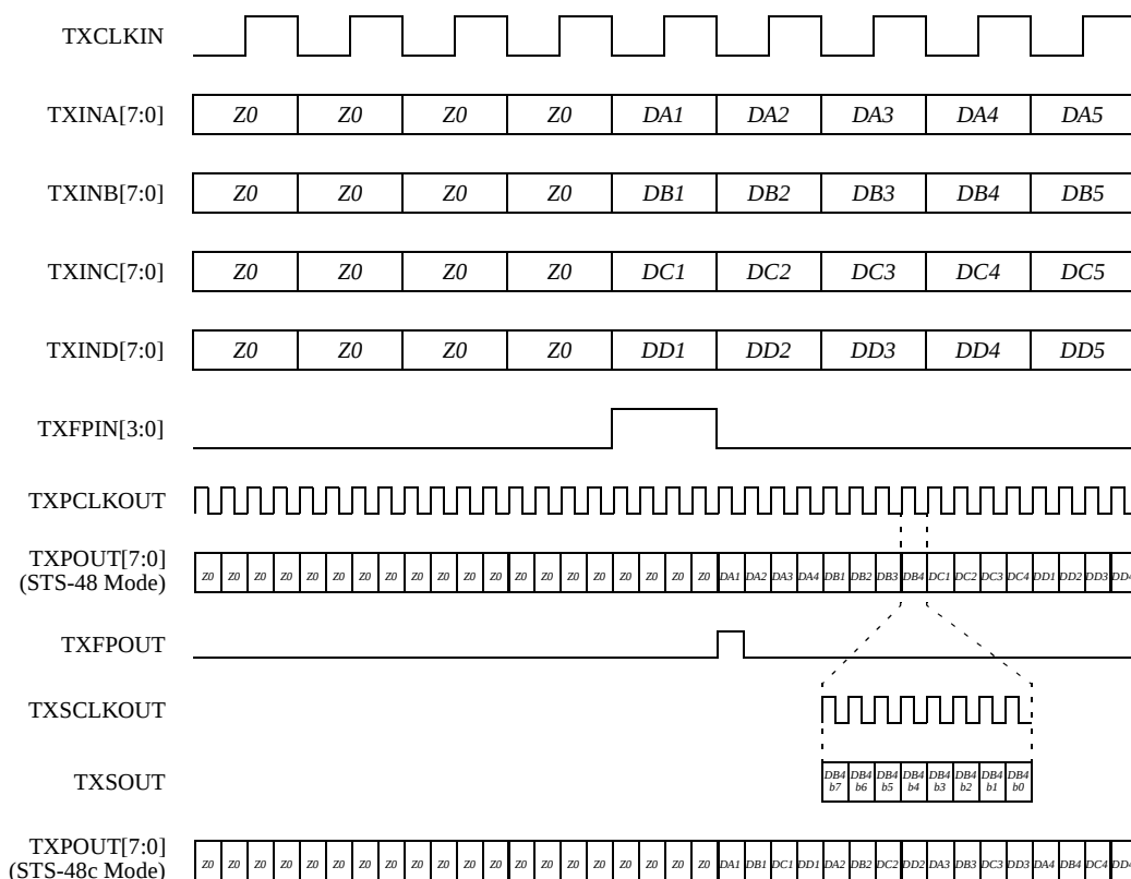
Figure 2: VSC8023 Functional Timing Diagram
