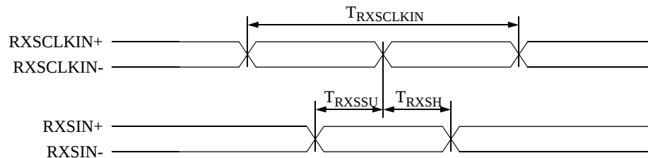
Figure 17: VSC8024 Serial Data Input Timing Diagram
