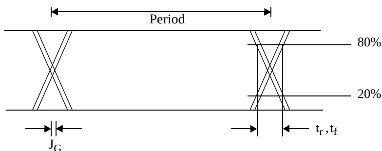
Figure 2: Re-timed Serial Output Data Eye Diagram
