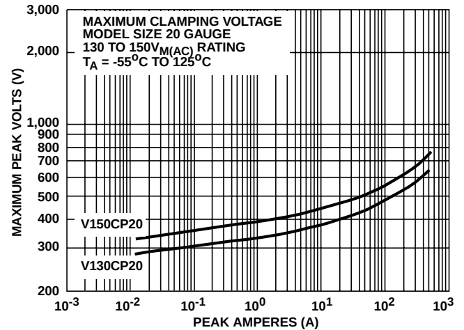
FIGURE 6. CLAMPING VOLTAGE FOR V130CP20 - V150CP20
