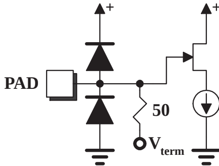
PECL Input Equivalent Circuit
