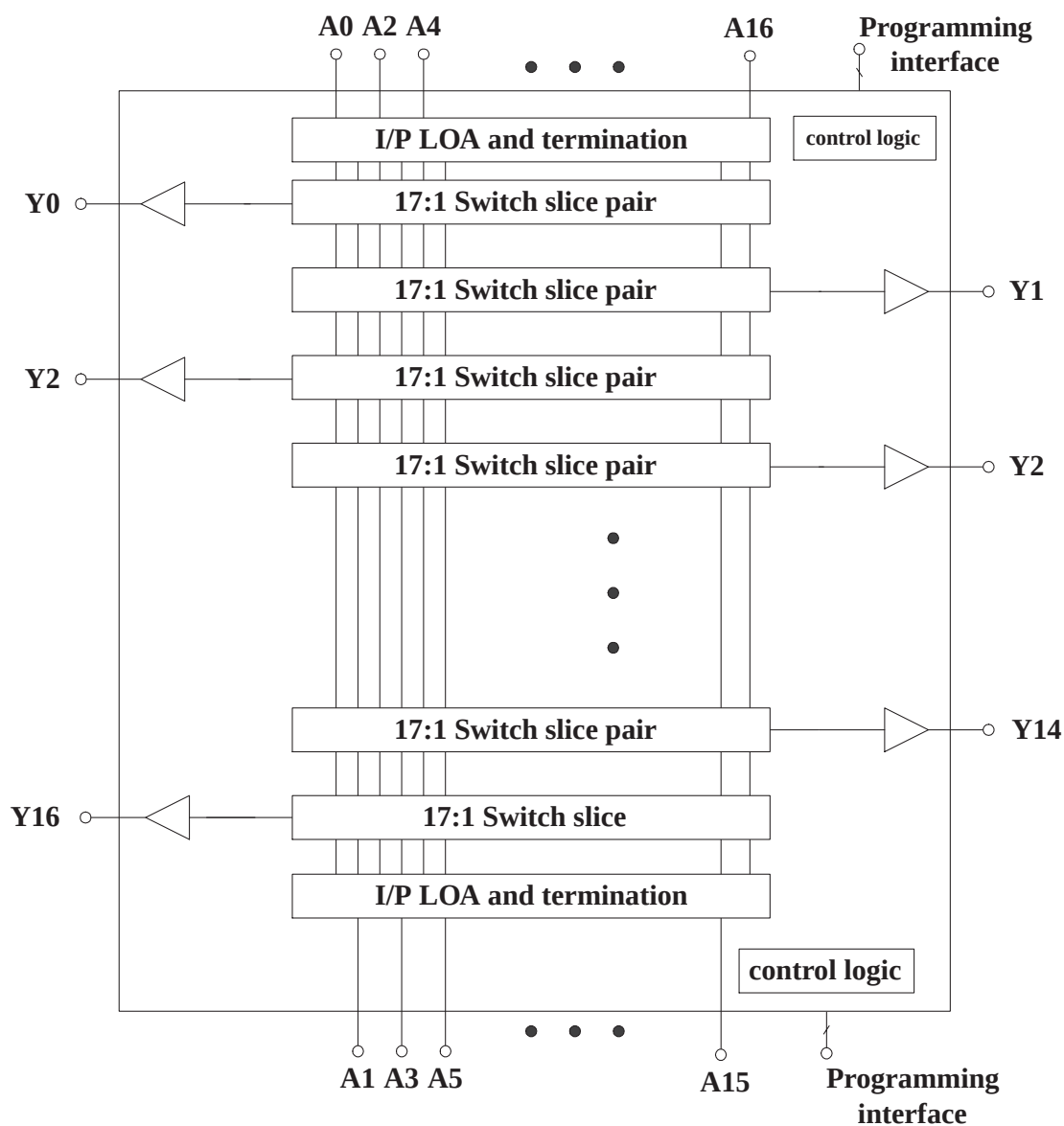
Figure 5: Functional Pinout Floorplan
