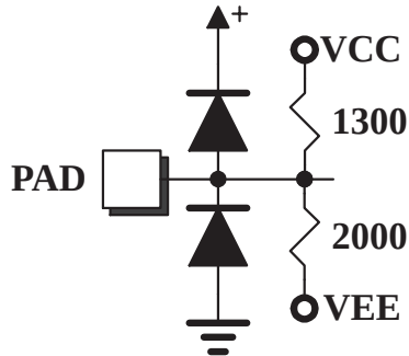
VCOM (L or R) Input Equivalent Circuit
