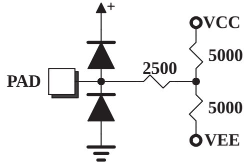
VHYS Input Equivalent Circuit
