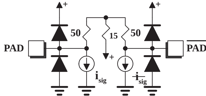
PECL Output Equivalent Circuit
