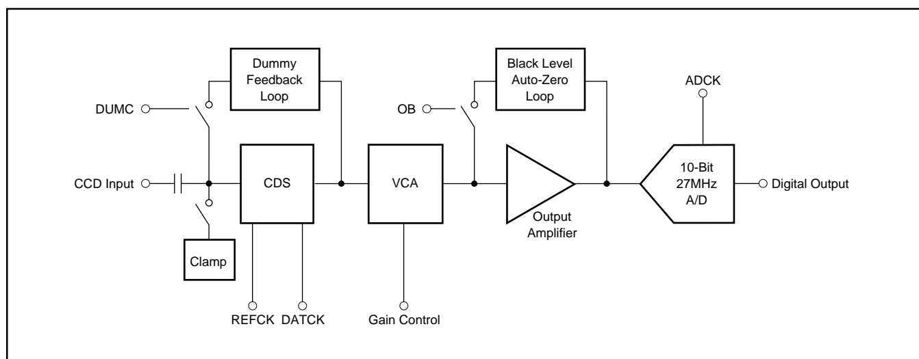
FIGURE 1. Simplified Block Diagram of VSP2100.
